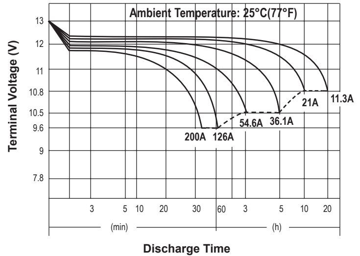
Discharge Characteristics
